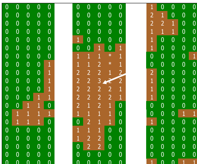
7. Examining the rate of disease spread from a point source in the centre of the plot.
